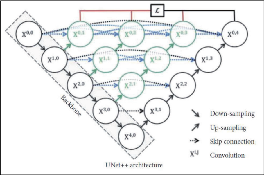
Supplementary Figure 1. U-Net++ deep learning architecture.
