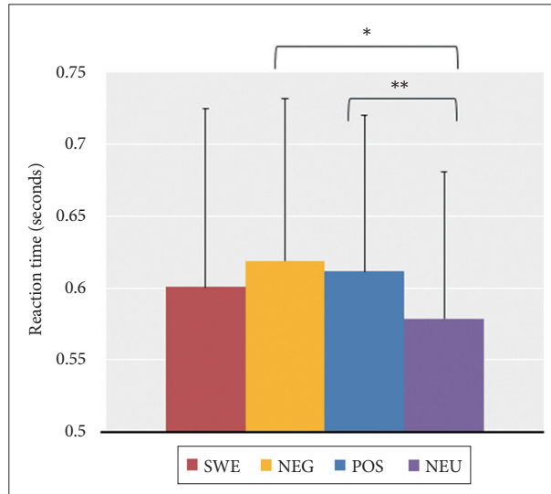
Supplementary Figure 2. The results of reaction time in emotional Stroop task. The trial effect on reaction time was significant [ F(3, 60)=5.518, p=0.002 ]. The differences between NEG, POS and NEU were significant after Bonferroni correction [ t(21)=3.356, *p=0.003 and t(21)=4.030, **p=0.001 , respectively]. Also, SWE trial showed a trend level difference compared to the NEU [ t(21)=2.323, p=0.046>0.05/6 ]. There was no significant difference between emotional stimuli (SWE, NEG, and POS). SWE: swearing, NEG: negative, POS: positive, NEU: neutral word.
