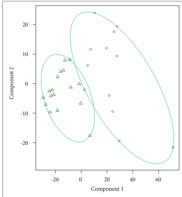
Supplementary Figure 1. The cluster plot using 'fpc' package of R. Our data was divided into two groups. All peer verbal abuse questionnaire (VAQ) scores \geq 40 was assigned to one group, except one subject (peer VAQ=40, parental VAQ=31). The two groups explain 100% of the point variability.
